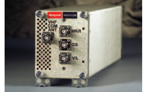
Nav-comm radio
